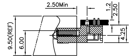
MATING DRAWING
